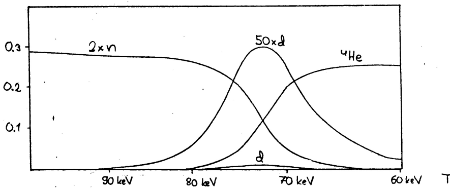
Figure 2: The time evolution of the n , {}^2\text{H} (written as d ) and {}^4\text{He} abundances during BBN. Notice how the final {}^4\text{He} abundance is determined by the n abundance before nuclear reactions begin. Only a small part of the neutrons decay or end up in other nuclei. Before becoming {}^4\text{He} , all neutrons pass through {}^2\text{H} . To improve the visibility of the deuterium curve, we have plotted it also as multiplied by a factor of 50. The other abundances (except p ) remain so low, that to see them the figure should be redrawn in logarithmic scale (see Fig. 4.3 of Kolb&Turner. This Figure is for \eta = 6 \times 10^{-10} . The time at T = (90, 80, 70, 60) keV is (152, 199, 266, 367) s. Thus the action peaks at about t = 4 min.
